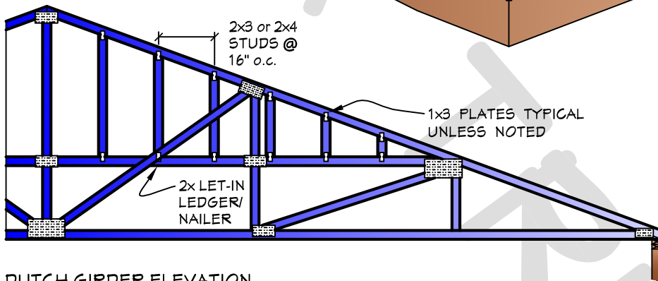
DUTCH GIRDER ELEVATION
